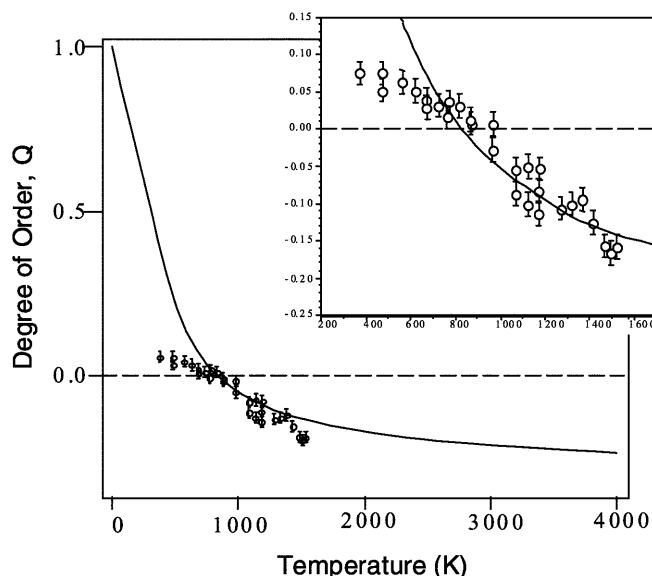
Fig. 7 Landau model for the non-convergent ordering in Fo50Fa50, incorporating the change from order to antiorder. The inset shows the fit over the range of the experimental data, suggesting that the data below around 800 K are not in equilibrium
