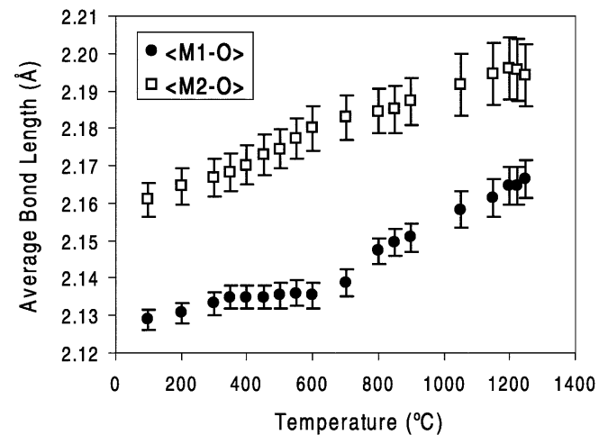
Fig. 4 Temperature dependence of the average bond lengths to oxygen at the M1 and M2 sites. The behaviour above and below about 630 °C ( T_{cr} ) shows different trends
