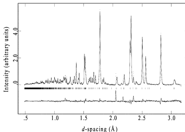
Fig. 1 Comparison of the experimental (dots) and calculated (solid line) neutron powder diffraction pattern for \text{MgFeSiO}_4 olivine at 600^\circ\text{C} , together with the difference plot (below) and expected peak positions (tick marks). The three peaks between 2.0 and 2.5 Å arise from the Vanadium furnace element
