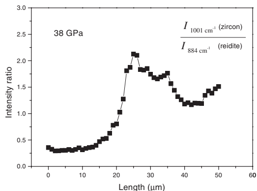
FIG. 5. Intensity ratio between the \nu_3 band near 1001 \text{ cm}^{-1} of the zircon remnants and the 884 \text{ cm}^{-1} band of the scheelite phase (38 GPa sample). The lines are visual guides.
