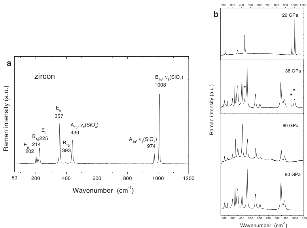
FIG. 3. Raman spectra of (a) zircon; (b) samples shocked at 20, 38, 60 and 80 GPa. The 20 GPa sample still has the zircon structure.
