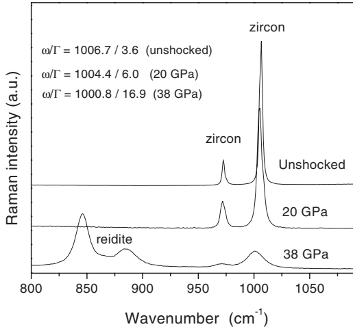
FIG. 6. The effect of high-pressure shock on the \nu_3 vibrations ( \text{SiO}_4 ) in zircon. The values of the frequency ( \omega in \text{cm}^{-1} ) and measured linewidth ( \Gamma in \text{cm}^{-1} ) of the \nu_3 vibration are given at different pressures.
