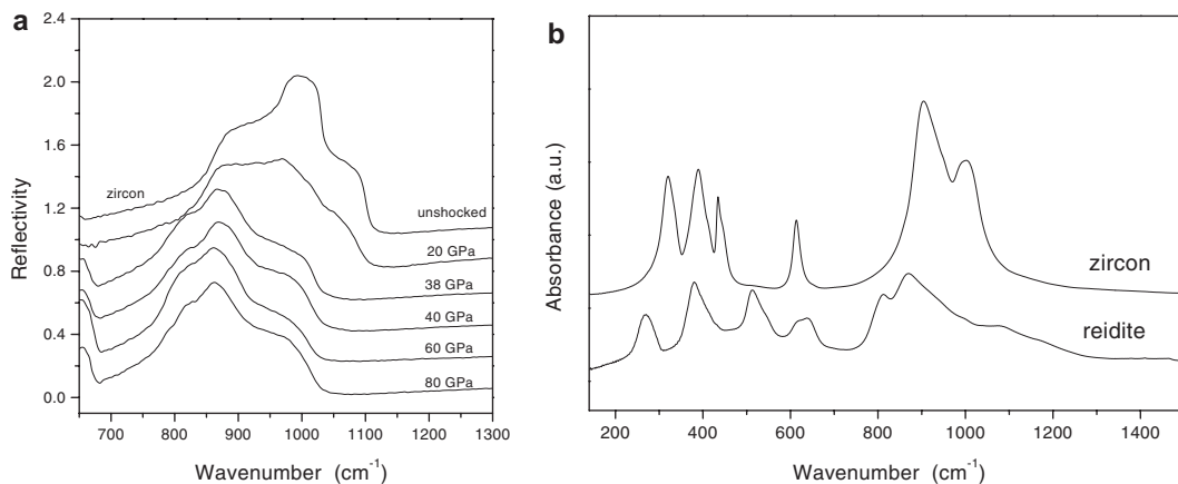
FIG. 1. (a). Micro-IR reflectance spectra ( 650\text{--}1300\text{ cm}^{-1} ) of the untreated zircon and the samples shocked at different pressures. Spectral differences between the untreated zircon and the samples shocked at and above 38 GPa are mainly due to the change of crystal symmetry during the zircon–reidite phase transition. (b) Comparison of IR powder absorption spectra of zircon and the sample shocked at 80 GPa containing mainly reidite phase ( 150\text{--}1500\text{ cm}^{-1} ).
