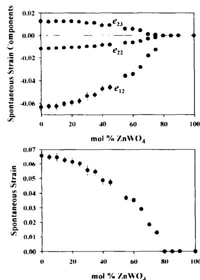
Fig. 4. Spontaneous strain components e_{12} , e_{22} and e_{23} and the scalar spontaneous strain, calculated from the equations of Redfern & Salje (1987), associated with the P2_1/c \rightarrow P1 structural phase transition.
