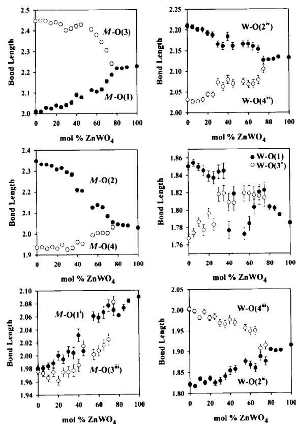
Fig. 7. Splitting of the M —O and W —O octahedral bond lengths (A) across the solid solution, indicating a large excess increase in the M —O(2) bond length due to the transformation from monoclinic to triclinic. Symmetry operators for text and figures: (i) 1-x, 1-y, 1-z ; (ii) -x, 1-y, 1-z ; (iii) 1-x, 1-y, -z ; (iv) x, y-1, z ; (v) x-1, y, z ; (vi) x-1, y-1, z .
