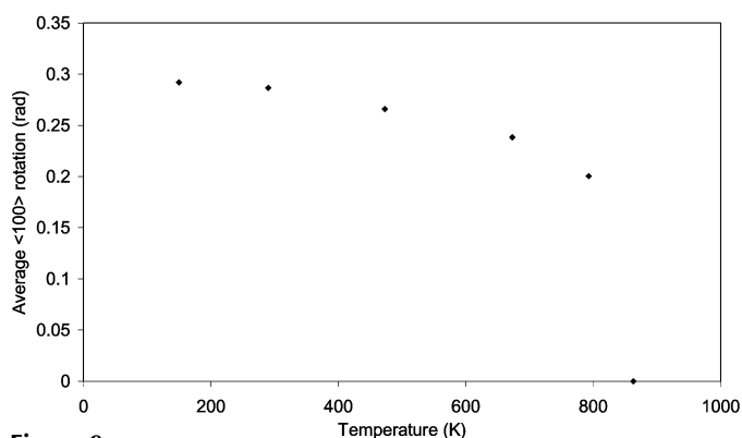
Figure 9 The average rotation of the polyhedra in an RMC configuration of quartz, relative to their positions in the ideal \beta phase. The rotation displays a dependence on the order parameter. Unfortunately the distribution of angles near the transition is so broad that the parameter cannot be obtained with any accuracy in this region.
