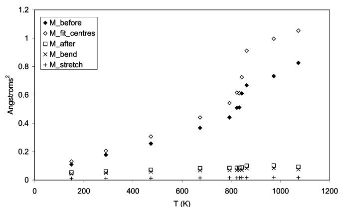
Figure 3 Average mismatch scores, M , in \text{\AA}^2 per polyhedron, for quartz. At each temperature, we are comparing one RMC configuration with another, where both configurations are fitted to the same data. The difference between the disorder M_{\text{before}} and the tetrahedral distortion M_{\text{after}} is due to rigid-unit motion. Since the disorder is much greater than the distortion, the dynamic disorder in quartz is largely accounted for by rigid-unit motions of the tetrahedra.
