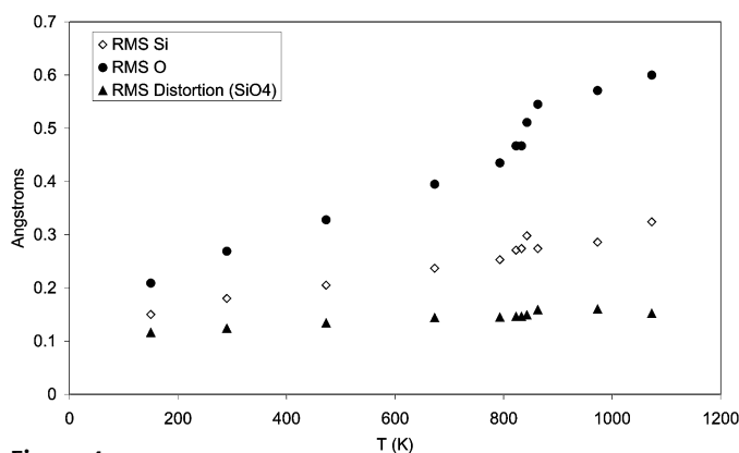
Figure 4 The mismatch values for quartz, interpreted as r.m.s. motions of O and Si atoms, and r.m.s. distortion of \text{SiO}_4 polyhedra. It is clear that the vertex O atoms are far more mobile than the Si atoms, as we would expect from rigid-unit motion. The r.m.s. distortion (distance of O atoms from geometrically ideal vertices) lies well below the r.m.s. motion of O atoms, indicating that RUMs make a dominant contribution to the amplitude of the dynamic disorder.
