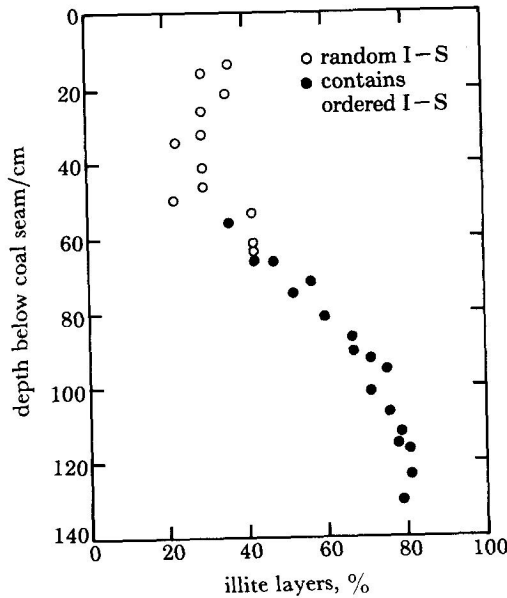
FIGURE 12. Relation between depth below coal, percentage illite layers in illite-smectite and type of interlayering for the under 2 \mu\text{m} size fraction of an Illinois underclay (after Rimmer & Eberl 1982).
